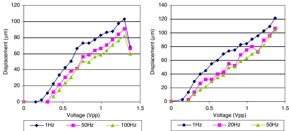
Figure 12. Left: non-trenched MetalMUMPs actuator voltage versus displacement curves. As actuation frequency increases, the amplitude of displacement decreases. Right: trenched MetalMUMPs actuator voltage versus displacement curves. Note that the frequencies used for the trenched actuators are lower than the non-trenched actuators.
