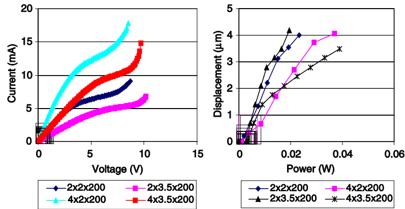
Figure 5. Left: I - V curves of PolyMUMPs actuators. All beams are 2\ \mu\text{m} wide, 200\ \mu\text{m} -long and 2 or 3.5\ \mu\text{m} thick. The 3.5\ \mu\text{m} thick actuators carry less current for the same applied voltage than the 2\ \mu\text{m} actuators due to the insulating thin oxide layer between the Poly1 and Poly2 layers. Right: power versus displacement curves of the PolyMUMPs bi-directional actuators.
