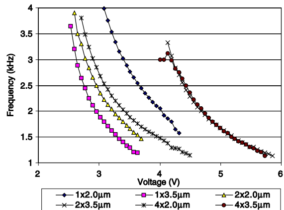
Figure 7. Maximum bi-directional operating frequency versus input voltage of PolyMUMPs surface-micromachined actuators.
