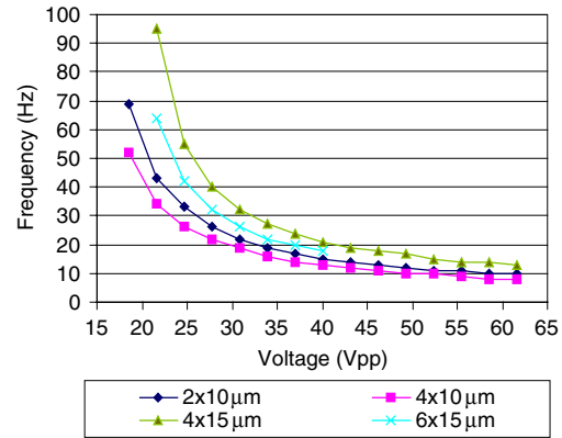
Figure 10. Maximum bi-directional operating frequency versus actuation voltage of 50 μm thick SOI actuators.
