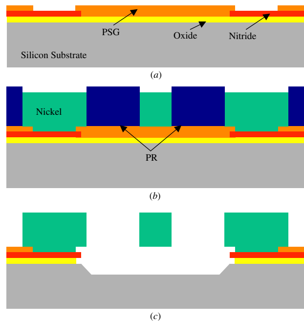
Figure 3. Key steps in MetalMUMPs to make trenched actuators. (a) Deposit 2 \mu\text{m} isolation oxide, 0.7 \mu\text{m} silicon nitride; pattern nitride to create trench area; deposit 1 \mu\text{m} PSG, pattern PSG. (b) Blank deposit of seed layer; deposit and pattern PR mold; electroplate 20 \mu\text{m} nickel and 0.5 \mu\text{m} gold (not shown) structural layer. Nickel on top of nitride would be anchored to the substrate, while nickel plated on top of PSG will be suspended after release. (c) Remove PR; release structures using HF. Etch 25 \mu\text{m} trench into the silicon substrate using KOH.
