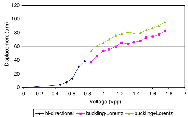
Figure 13. Voltage versus displacement measurements for MetalMUMPs actuators before and after permanent deformation at around 40 \mu\text{m} of displacement. The amplitude of movement alternates between high and low states with a difference of several microns due to the Lorentz force in two opposite directions.
