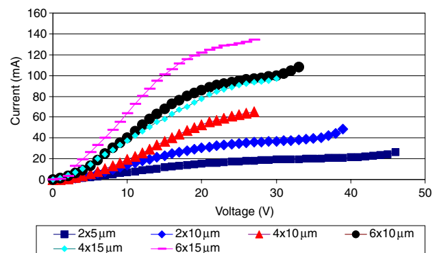
Figure 8. I - V characteristics of SOI bi-directional actuators.
