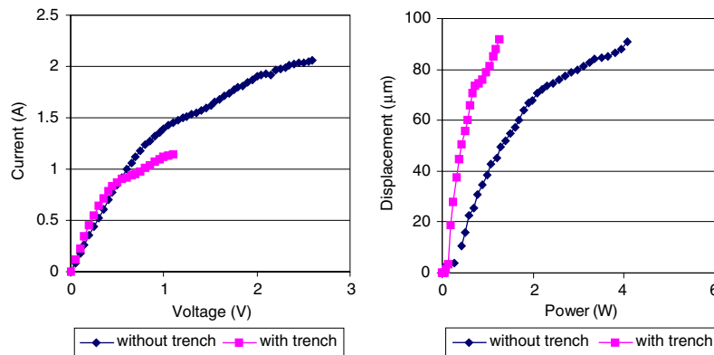
Figure 11. Left: I-V curve of trenched and non-trenched MetalMUMPs bi-directional actuator. Right: power versus displacement curve of MetalMUMPs bi-directional actuators.
