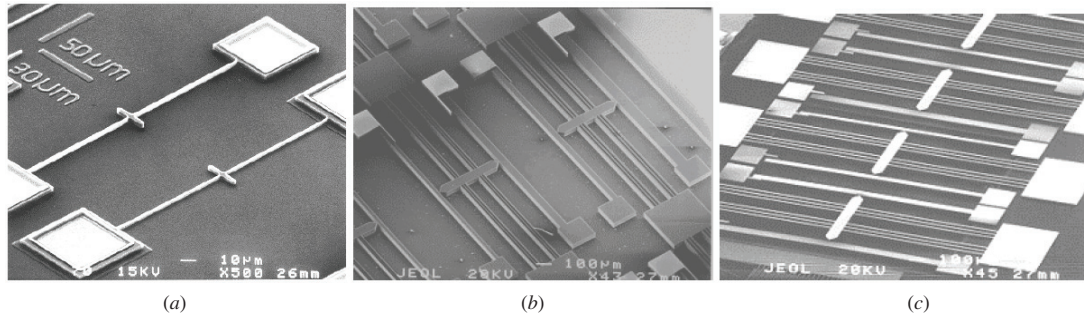
Figure 2. SEM micrographs of (a) two single-beam bi-directional actuators made using the PolyMUMPs process. The top actuator is 3.5 \mu\text{m} in thickness; the bottom actuator is 2 \mu\text{m} in thickness. (b) Actuators made using a 50 \mu\text{m} thick SOI process with a 1 \mu\text{m} thick buried oxide layer. These actuators have an actuation beam length of 2000 \mu\text{m} and widths ranging from 5 to 15 \mu\text{m} . (c) MetalMUMPs bi-directional actuators.
