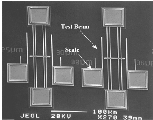
Figure 4. SEM of PolyMUMPs bi-directional actuators and their force testing structure. These 200 \mu\text{m} long, 2 \mu\text{m} wide and 3.5 \mu\text{m} thick actuators have four actuation beams. A bi-directional displacement of 3.5 \mu\text{m} could be achieved under 4 V and 10 mA and the maximum measured force output is 200 \mu\text{N} .
