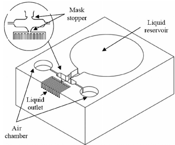
Figure 2. Schematic diagram of the flow discretizer.
