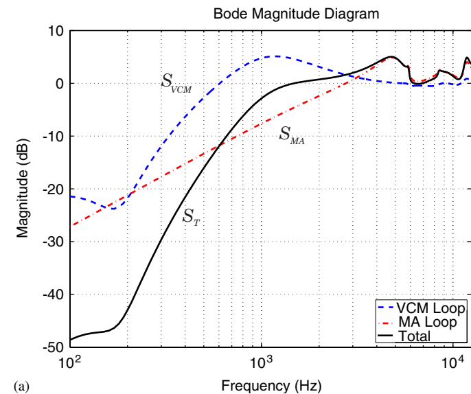
Fig. 7. (a) Bode plots of simulated sensitivity transfer functions S_{VCM}(z) , S_{MA}(z) and S_T(z) ; (b) Bode plots of the simulated (dashed) and experimentally measured sensitivity transfer function S_T(z) .
