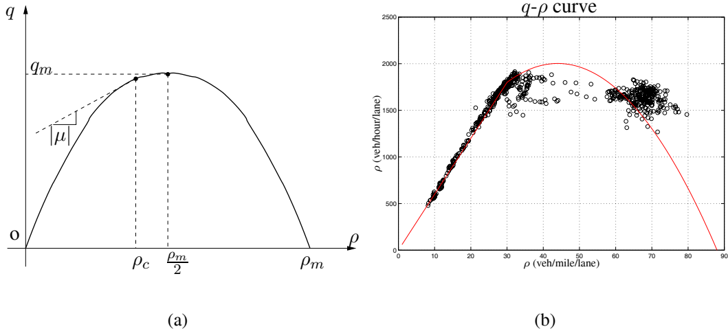
Figure 3: Flow-density relationship ( q - \rho curve) (a) VTG policy as Eq. (42); (b) traffic data of highway I-210 (dot) and fitting curve (solid).
