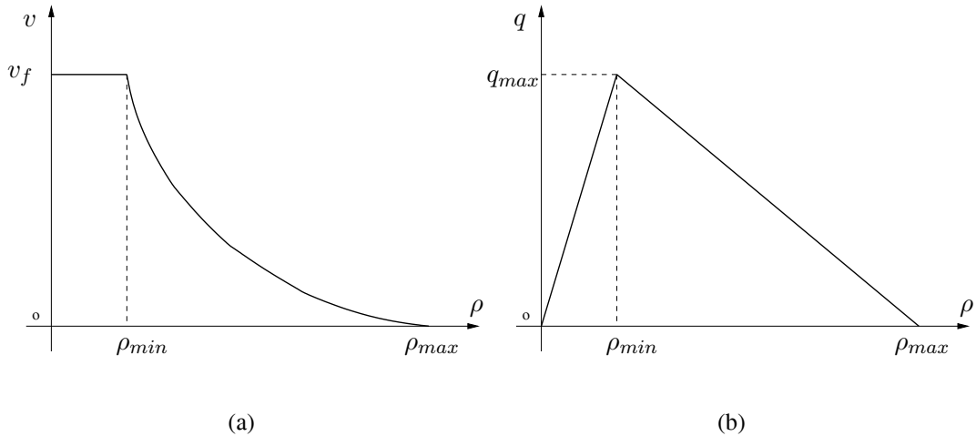
Figure 1: A schematic of the CTH policy (a) velocity-density relationship ( v - \rho curve); (b) flow-density relationship ( q - \rho curve).
