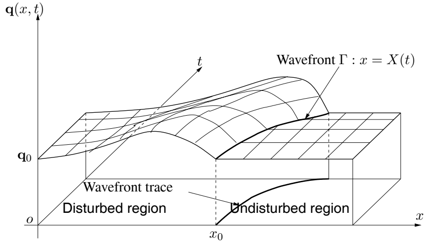
Figure 2: A schematic of a solution surface, wavefront and wavefront trace with an initial C^1 discontinuous condition \mathbf{q}(x_0, 0) .
