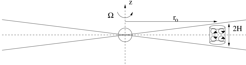
FIGURE 2. Side view of Keplerian disk with anticyclone. The disk is believed to be “flared”, with scale height H increasing with radius. The anticyclone fills the disk in the vertical direction.
